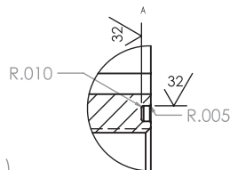
DETAIL C SCALE 2 : 1
